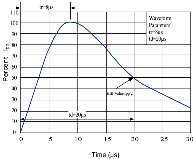
Figure 5: Pulse Waveform
